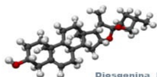
Diosgenina
